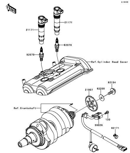
C-14 Ignition System
