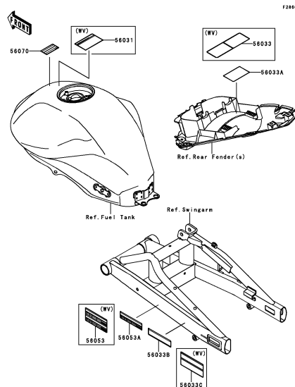
G-10 Labels
