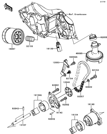
C-12 Oil Pump
