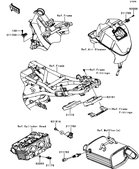
C-11 Fuel Injection
