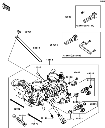
C-9 Throttle
