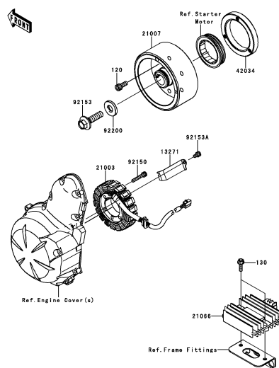
C-13 Generator
