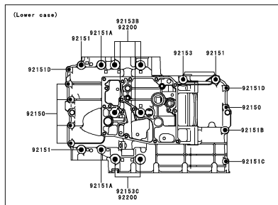
C-6 Crankcase Bolt Pattern
