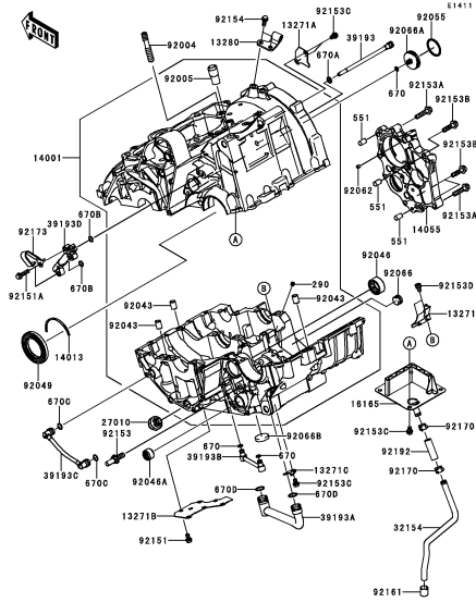
C-4 Crankcase(1/2)
