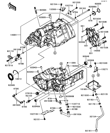
C-5 Crankcase(2/2)
